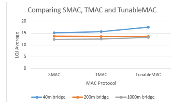
Fig. 8. Comparing LQI for SMAC, TMAC and TunableMAC
