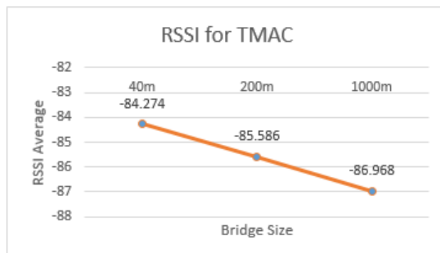
Fig. 3. RSSI for TMAC under three network sizes
