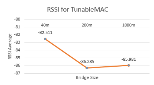
Fig. 5. RSSI for TunableMAC under three bridge sizes
