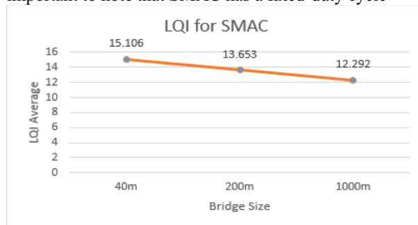
Fig. 2. LQI for SMAC under three network sizes
