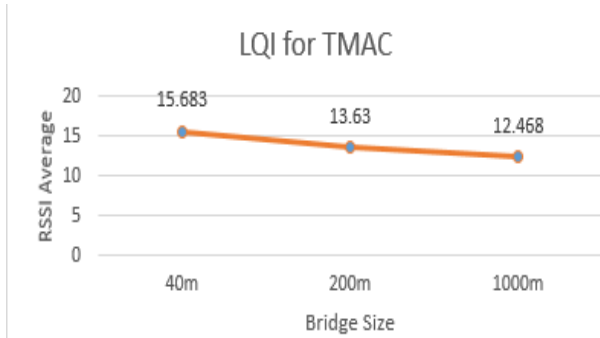
Fig. 4. LQI for TMAC under three network sizes
