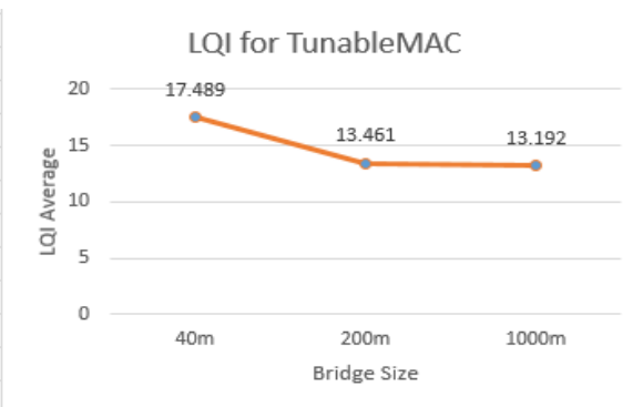
Fig. 6. LQI for TunableMAC under different bridge sizes
